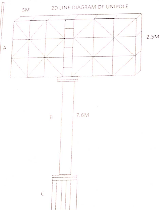
FOUNDATION MS STRUCTURE 7.5'(H)X2.5'X2.5
