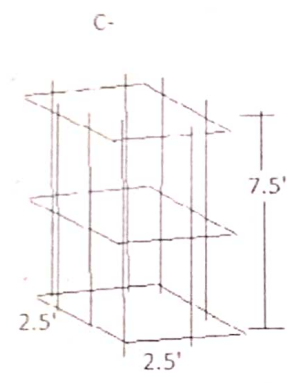
FOUNDATION MS STRUCTURE 7.5'(H)X2.5'X2.5
